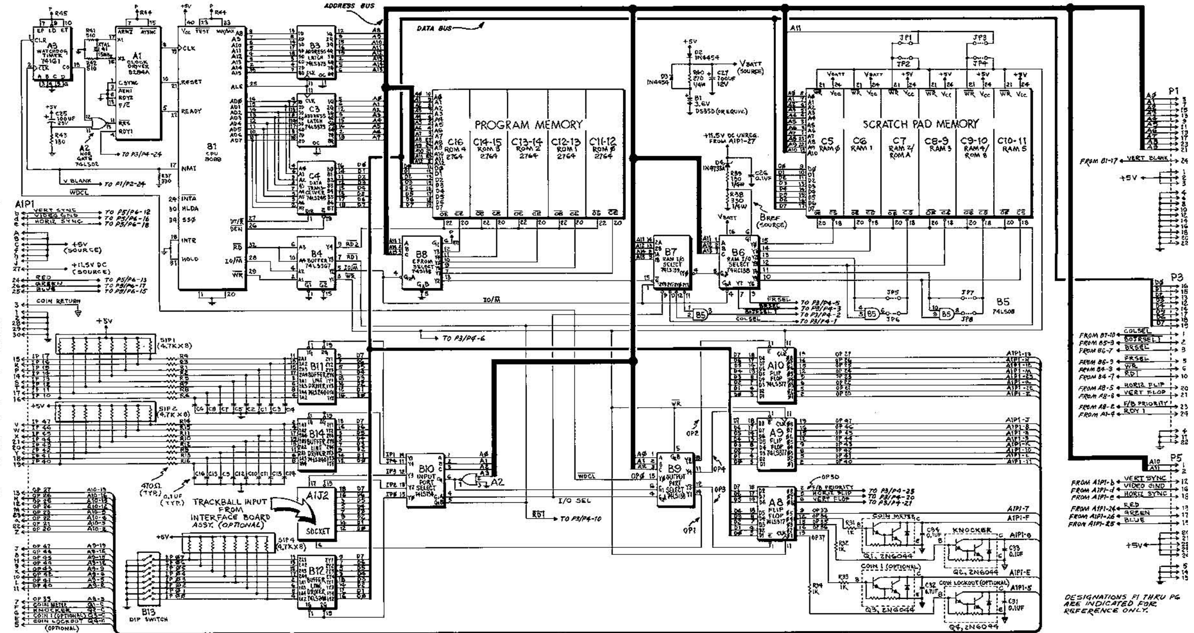
LOGIC BOARD ASSY. (A1), SCHEMATIC DIAGRAM, SHEET 1 OF 1
